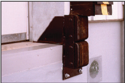
Vertical laminated bumpers with gusseted bracket and load distribution plate.
